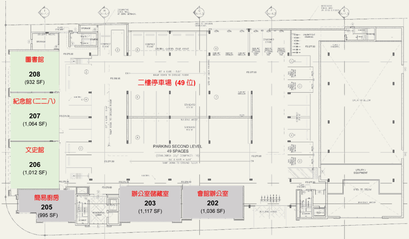
2ND FLOOR / PARKING SECOND LEVEL PLAN SCALE: 1" = 10'-0"
