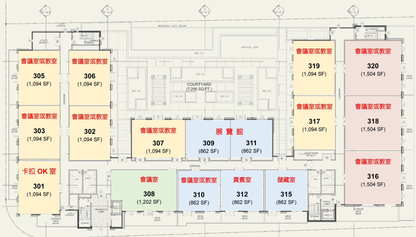
THIRD FLOOR PLAN SCALE: 1" = 10'-0"
